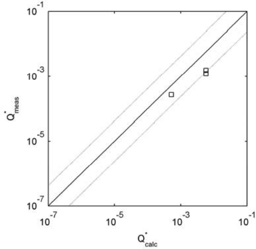
Figure 7: Evaluation of present overtopping formula against data by Kuhnen (2000).
