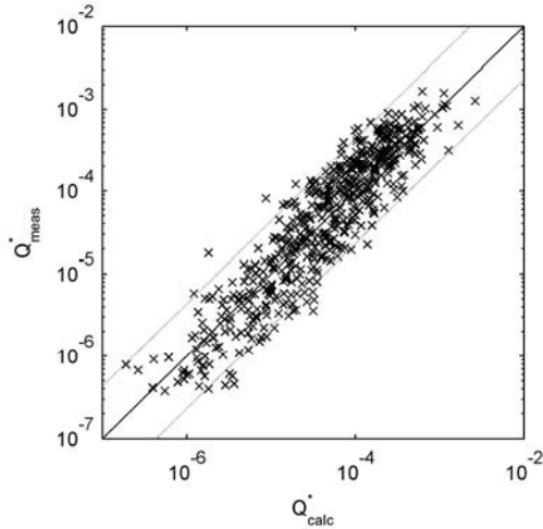
Figure 9: Evaluation of present overtopping formula against data by Lykke Andersen & Burcharth (2004).
