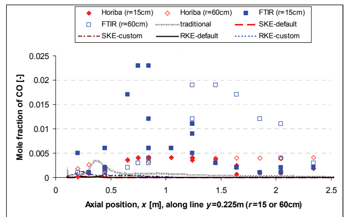
Fig. 4 CFD vs. measurements on line y=0.225m
