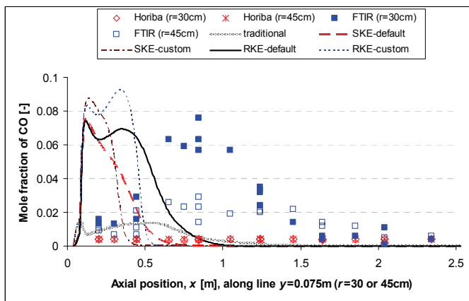
Fig. 3 CFD vs. measurements on line y=0.075m
