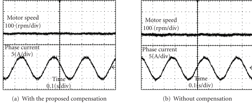
FIGURE 3: Experimental result of current control at 100 rpm (speed and phase current).
