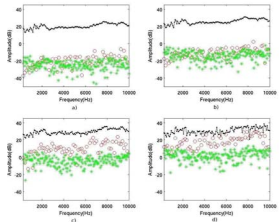
Fig. 9: Output spectrum of the teleconferencing loudspeaker at RMS input signal a) 0.02, b) 0.04, c) 0.08, d) 0.16
