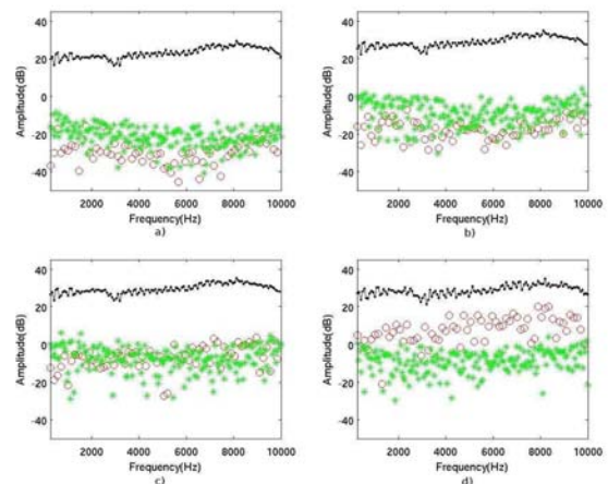
Fig. 10: Output spectrum of the studio monitor at RMS input signal a) 0.02, b) 0.04, c) 0.08, d) 0.16
