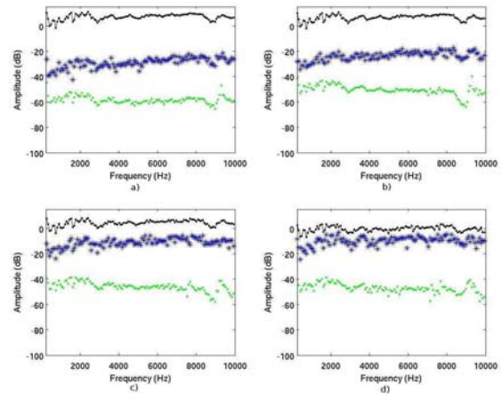
Fig. 5: \hat{G}_{BLA} , nonlinear distortion and noise level of the teleconferencing loudspeaker at RMS input signal a) 0.02, b) 0.04, c) 0.08, d) 0.16
