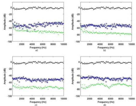
Fig. 6: \hat{G}_{BLA} , nonlinear distortion and noise level of the studio monitor at RMS input signal a) 0.02, b) 0.04, c) 0.08, d) 0.16
