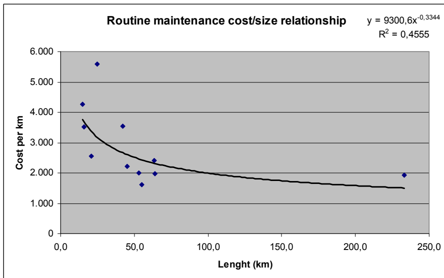
Figure A-4. Cost/size relationships in routine maintenance of 2L highways in Uganda (based on data from the World Bank, 2002).
