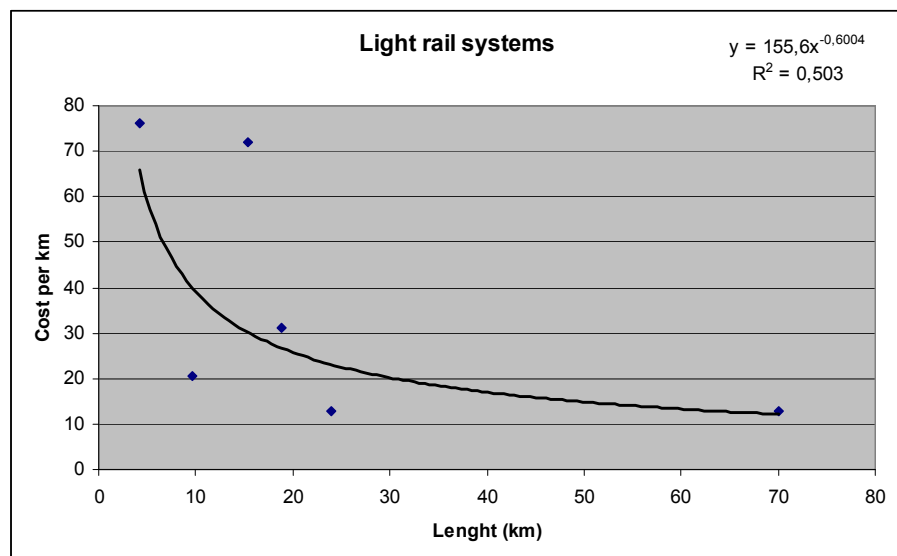
Figure A-8. Cost/size relationships for light rail systems (based on data from Railway Technical Web Pages).
