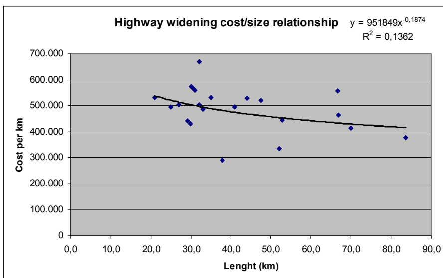
Figure A-5. Cost/size relationships in highway widening projects in Thailand (based on data from the World Bank, 2002).
