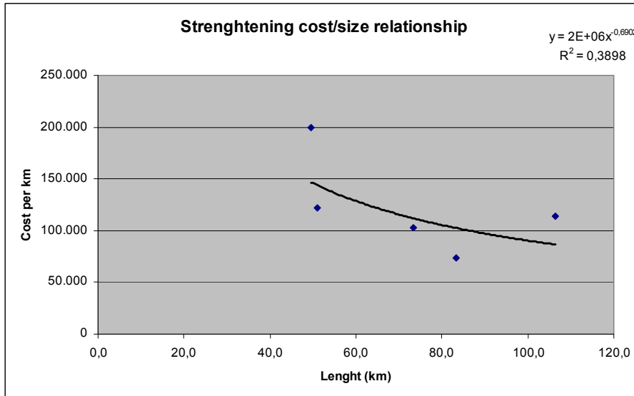
Figure A-3. Cost/size relationships in strengthening roads in Bangladesh (based on data from the World Bank, 2002).
