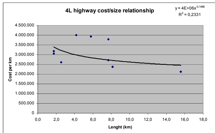
Figure A-2. Cost/size relationships in construction of new 4L highways in Poland (based on data from the World Bank, 2002).
