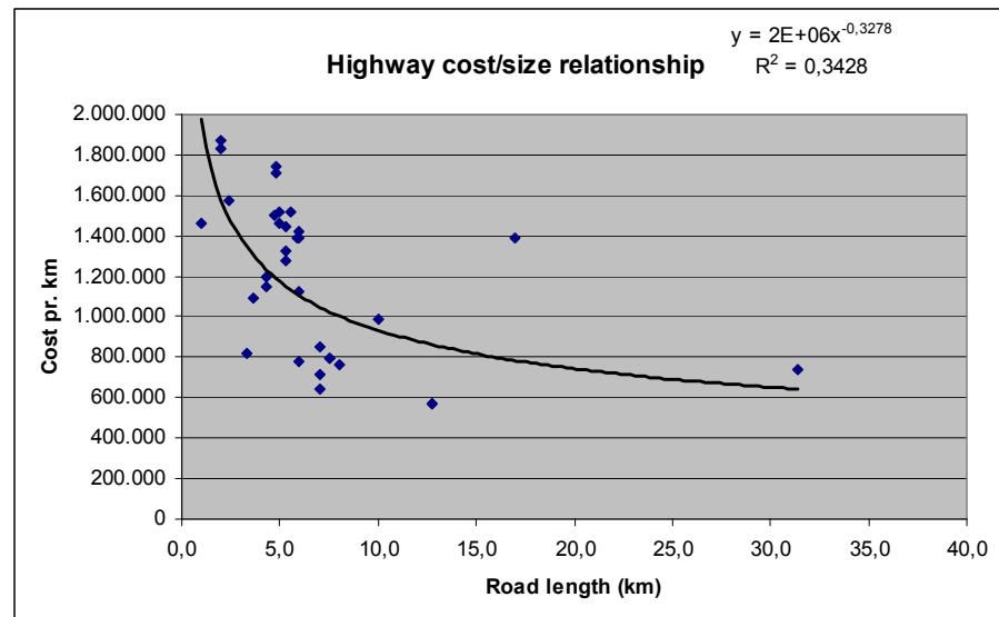
Figure A-1. Cost/size relationships in construction of new 2L highways in Poland (based on data from the World Bank, 2002).
