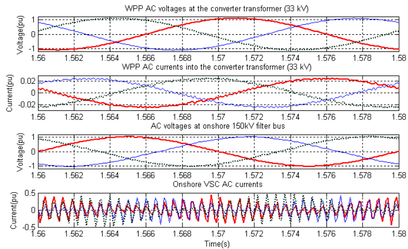
Fig. 7 Steady state operation at no load
