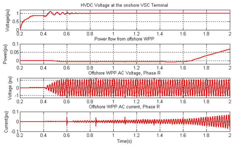
Fig. 6 Charging VSC-HVDC and energizing the offshore grid
