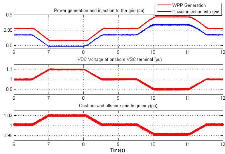
Fig. 9 WPP response to onshore grid frequency variation
