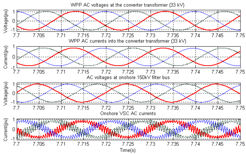
Fig. 8 Steady State operation at full 400MW WPP generation
