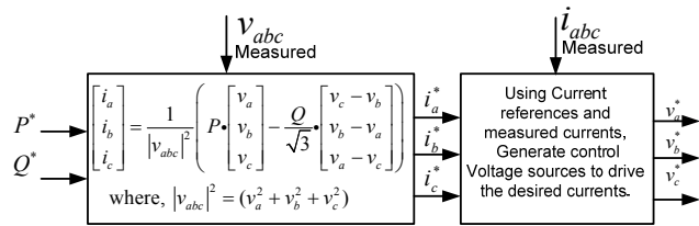
Fig. 3 Block Diagram of Onshore VSC Controller
