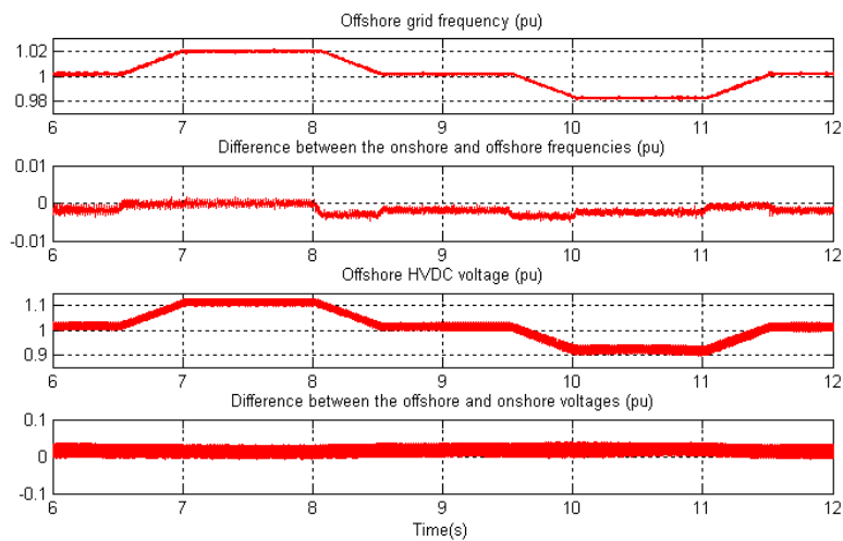
Fig. 10 Difference in voltages and frequencies measured onshore and offshore
