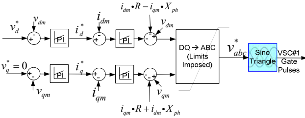
Fig. 2 Block Diagram of Offshore VSC Controller
