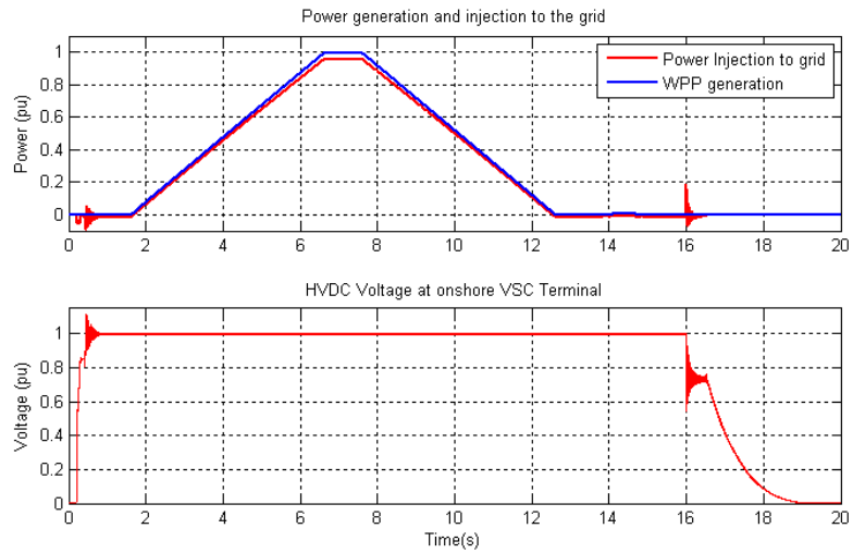
Fig. 5 WPP Power generation and injection into the onshore grid
