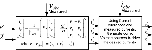
Fig. 3 Block Diagram of Onshore VSC Controller
