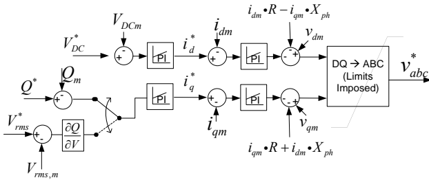
Fig. 3 Block Diagram of Onshore VSC Controller
