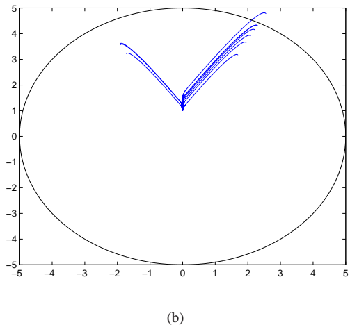
Fig. 4. (a) Two local solutions, one at (0, 1) and one at (0, 1.53) , of the local system governed by f_1 . (b) 10 realizations of X^{(0,1)1} .
