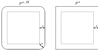
Fig. 1. P^{\epsilon, H} and P^\epsilon with P indicated by the dotted square.
