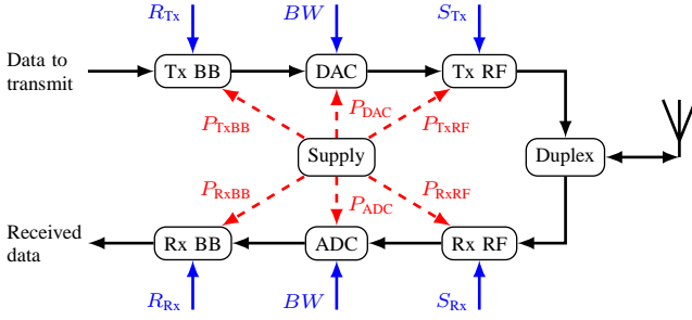
Fig. 1. LTE smartphone modem power model. Red dashed lines indicate power consumption and blue solid lines are input parameters.
