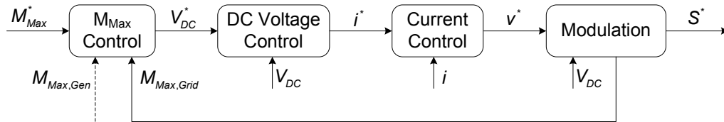
Figure 3: Proposed adaptive dc-link voltage controller
