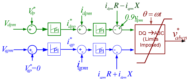
Fig. 4 Offshore VSC controller (positive sequence)
