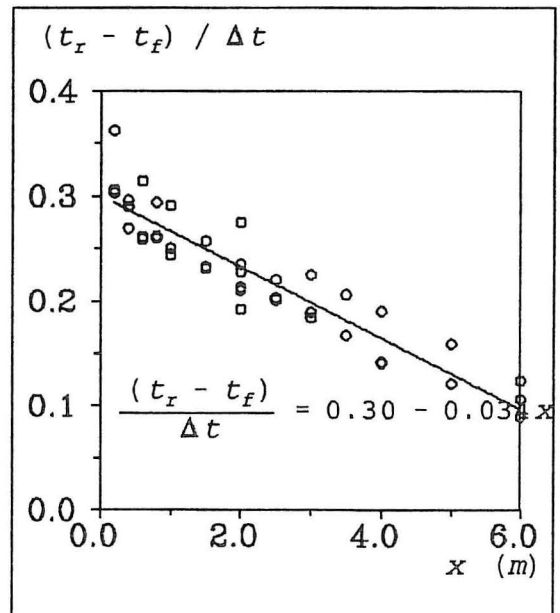
Fig. 6. Decay of temperature difference between the reference temperature and the minimum temperature in the airflow along the floor.
