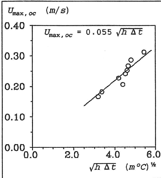
Fig. 1. Maximum velocity in the occupied zone as a function of height of the surface and temperature difference between surface and room.
