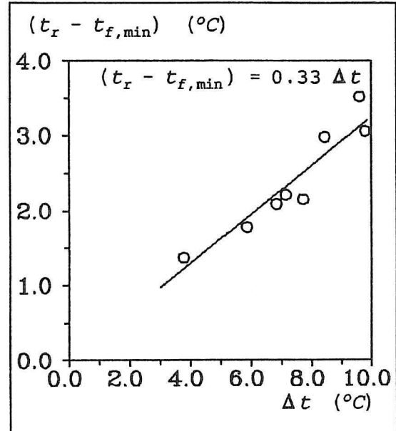
Fig. 2. Temperature difference (t_r - t_{f, \min}) as a function of the temperature difference \Delta t .
