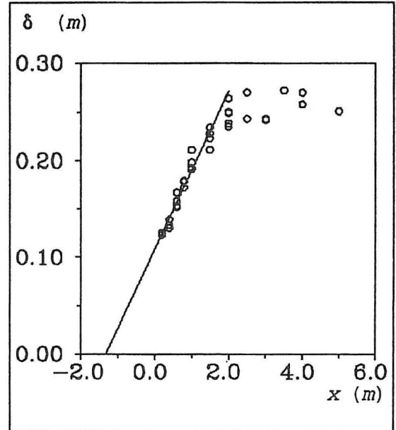
Fig. 4. Growth of thickness of the cold airflow region along the floor with distance from the cold vertical surface.
