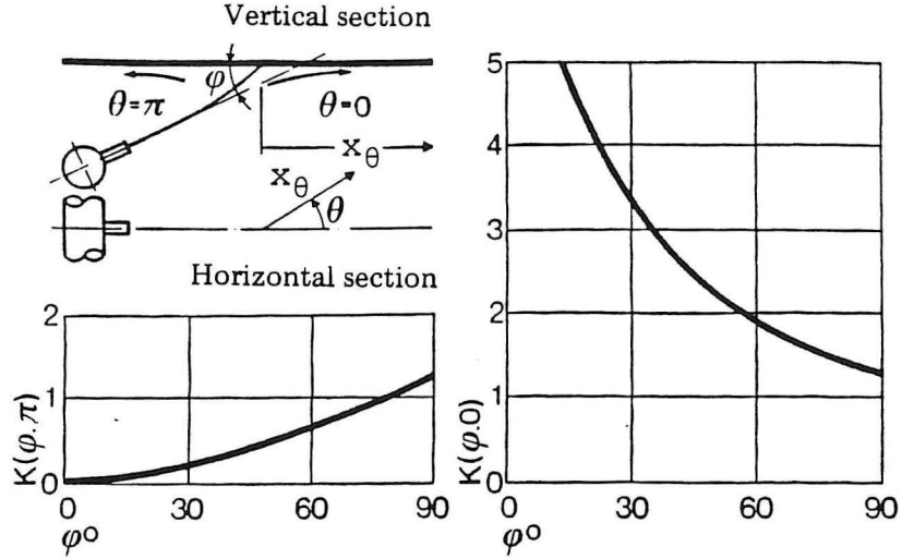
Figure 3. Oblique impinging jet. K(\varphi, \theta) is the coefficient in equation (1).
