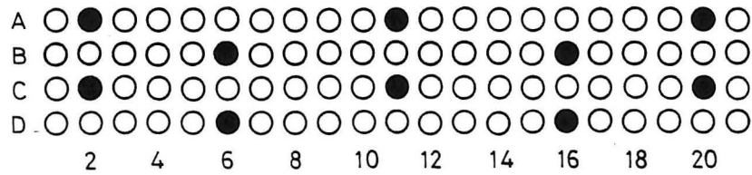
Figure 4. Location of 10 measuring points for measurement of the mean supply velocity.
