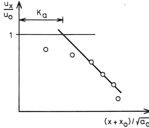
Figure 7. The velocity decay u_x/u_0 versus the distance (x + x_0)/\sqrt{a_0} in a double logarithmic coordinate system.
