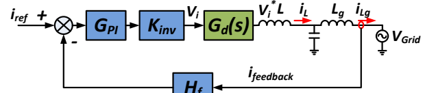
Fig. 7. Block diagram of the control loop.
