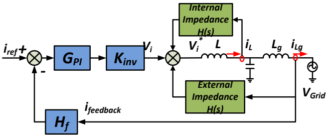
Fig. 13. Block diagram including the grid current feedback damping loop.
