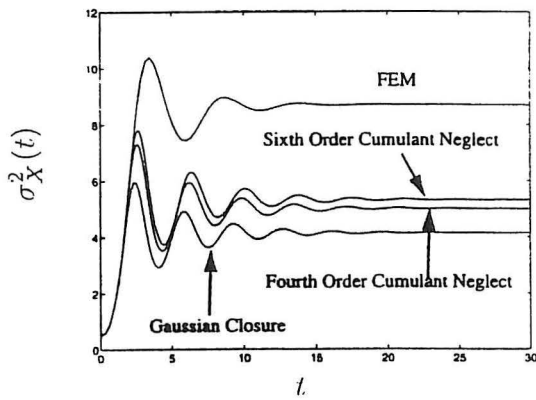
Figure 2. Non-stationary results. a) \sigma_X^2(t) versus time for 2nd, 4th, 6th order closure, Bergman et al. (1995). b) \sigma_X^2 versus time for modified 2nd order closure.
