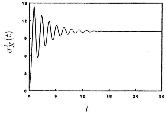
Figure 2. Non-stationary results. a) \sigma_X^2(t) versus time for 2nd, 4th, 6th order closure, Bergman et al. (1995). b) \sigma_X^2 versus time for modified 2nd order closure.
