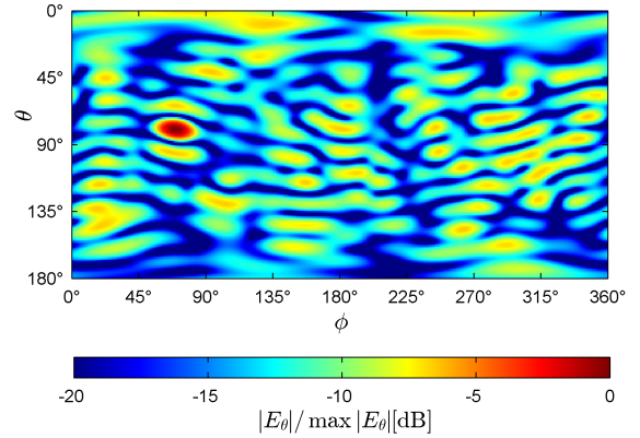
Figure 3: E-field radiation pattern with beam steered to \theta = 80^\circ , \phi = 70^\circ direction.
