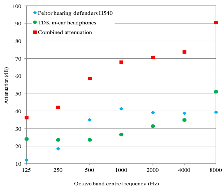
Figure 1. Attenuation provided by in-ear headphones, hearing defenders and the combination of the two.
