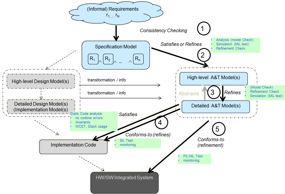
Figure 3: Main V&amp;V-flow.
