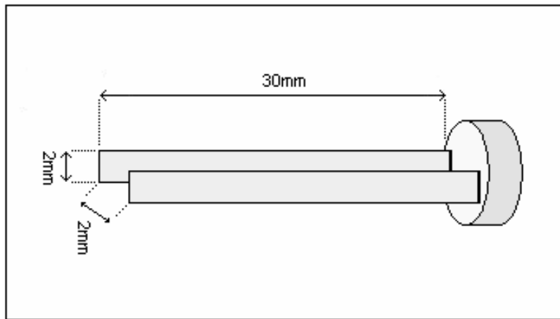
Figure 5: The diagram of the E.C. sensors.
