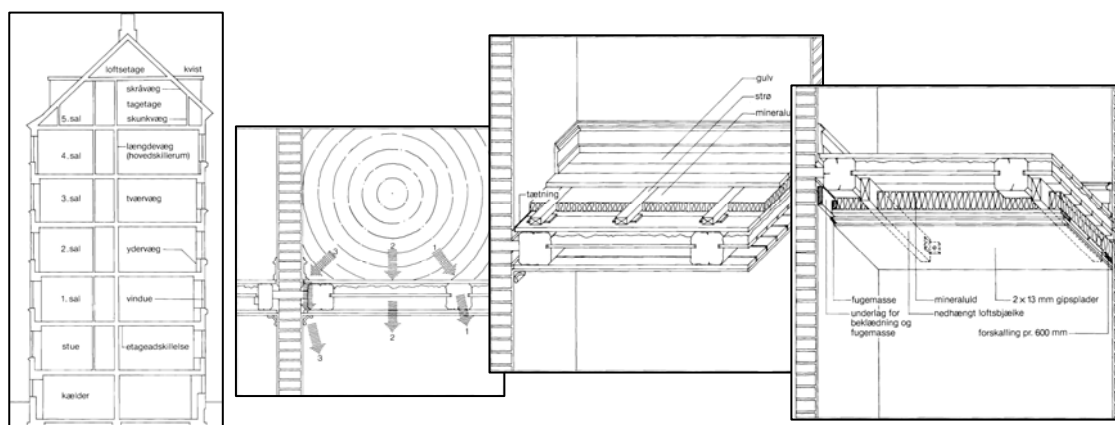
Figure 5. Examples on instructions for improvement of sound insulation of old housing. Source: SBi Guidelines 173, Sound insulation of buildings – Old buildings, 1992 (in Danish).
