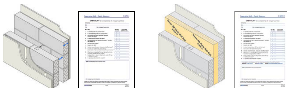
Figure 6. Examples construction details and related checklists from Robust Details [20].
