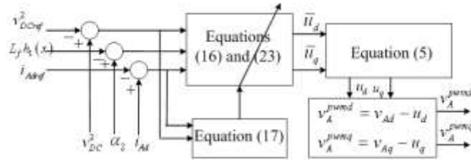
Fig. 5 Block diagram of the DC-link voltage control system of VSC1.
