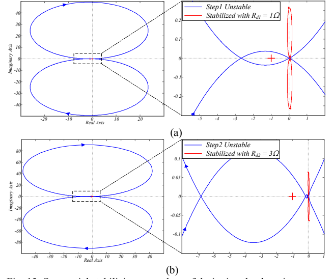
Fig. 13. Sequential stabilizing procedure of designing the damping resistor R_d to obtain stable two-inverter system in Fig. 11.
