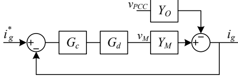
Fig. 6. Norton equivalent model for the grid-inverter with balanced load condition.
