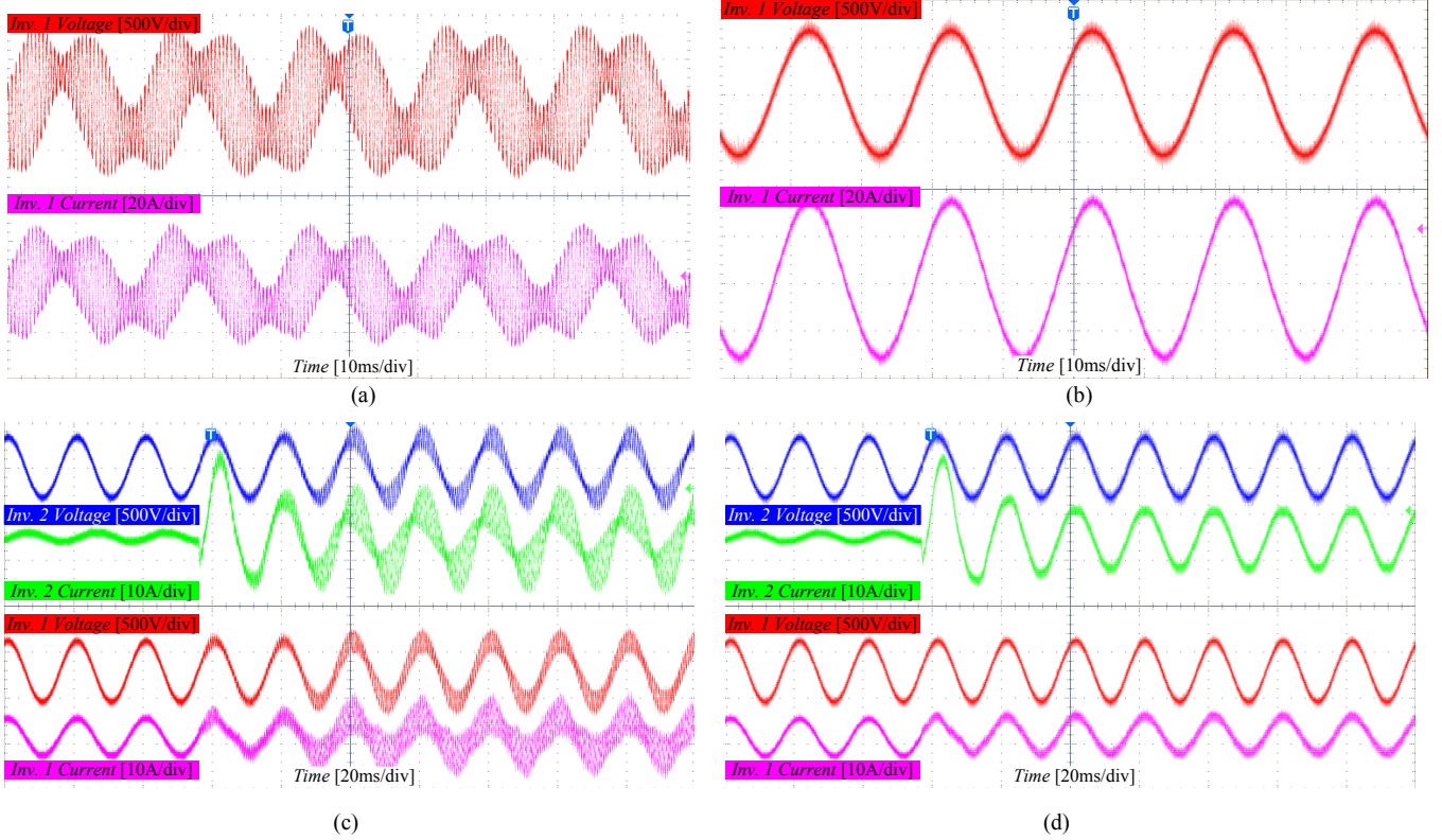
Fig. 13. Experimental waveforms using two paralleled inverters: a) Step 1 unstable case voltage and current; b) stabilized with passive damping of Inv. 1 with R_{d1} = 1 \Omega ; c) Step 2 unstable with the two inverters; d) stabilized with passive damping of Inv. 2 R_{d2} = 3 \Omega
