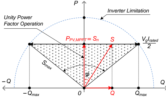
Fig. 5. PQ-diagram for a single-phase PV inverter.
