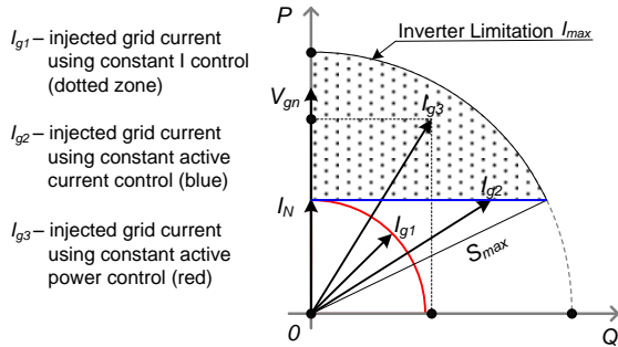
Fig. 7. Representations of the injected grid current using different control strategies considering the inverter current limitation.
