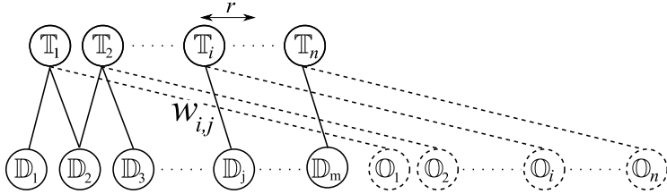
Fig. 2. Example of the bipartite graph that must be solved for each frame. Each tracker \mathbb{T}_i is connected to all detections \mathbb{D}_j that lie within its search radius and to one occlusion node \mathbb{O}_i .
