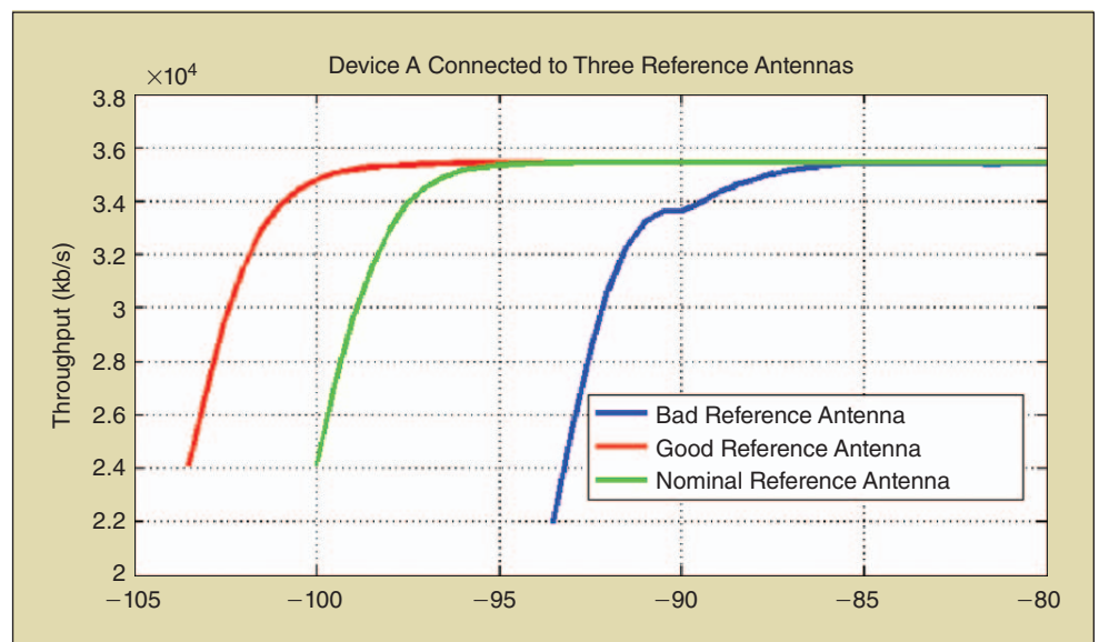
FIGURE 7 The measured throughput results of a mobile phone with three different reference antennas for the same spatial channel model.
