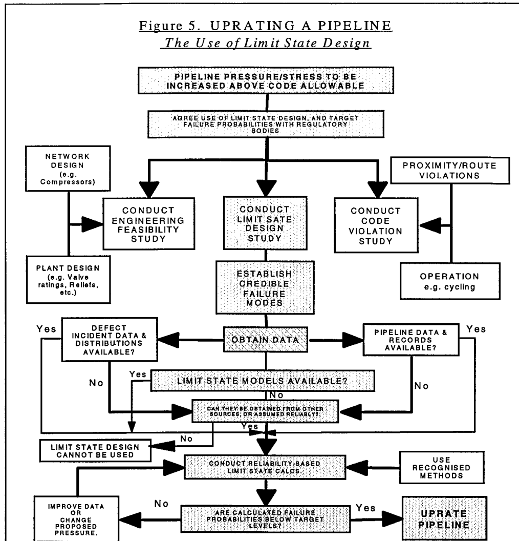
Figure 24. Updating of a pipeline (from [32]).
