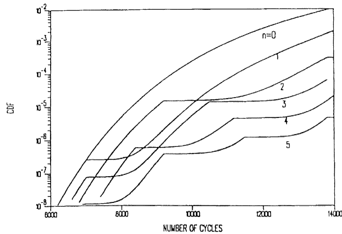
Figure 21. Cumulative probability of disfunction as a function of service life. Effect of ECI with different number of inspections n (from [30]).
