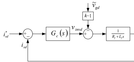
Fig. 5. Reduced current control block diagram with feedforward
