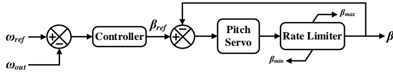
Fig. 5. Modified pitch angle control used in FSIG-based wind turbine.
