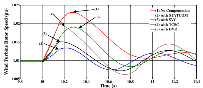
Fig. 31. FSIG rotor speed.
