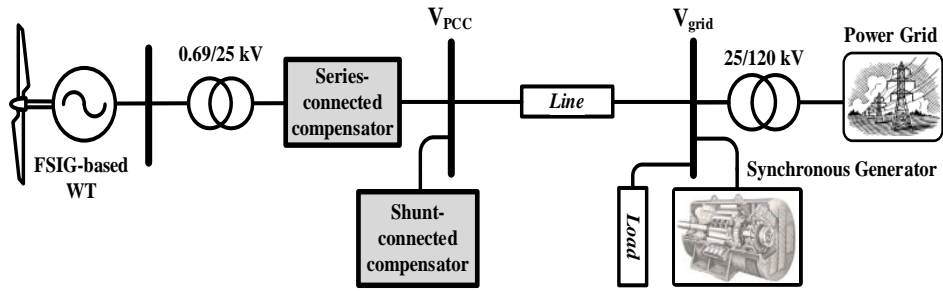
Fig. 26. Single-line diagram of the power network including a series-connected or shunt-connected compensator.
