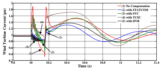
Fig. 30. Stator current of the FSIG.
