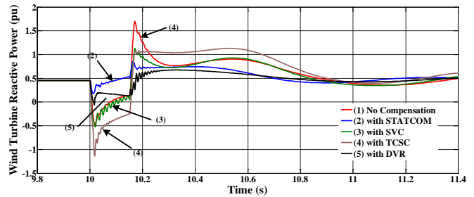
Fig. 29. Reactive power absorbed by FSIG.
