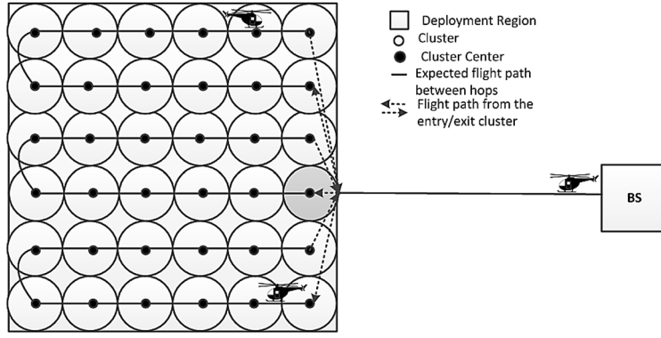
Fig. 2 Sensing region from top, path of DCFly [1]
