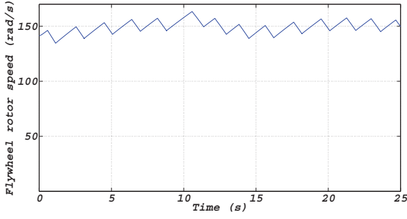
Fig. 5. Flywheel speed.
