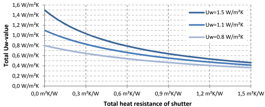
Figure 2. Calculated total U-values for the system of different glazing units with an insulation shutter, as function of the shutter heat resistance.
