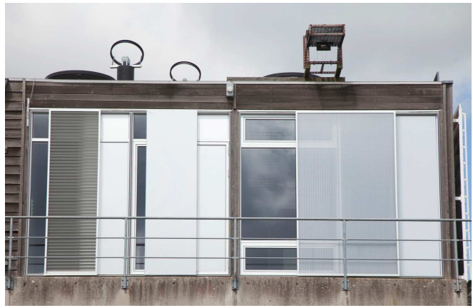
Figure 4. Three prototypes of Energy Frames elements were initially tested in the Daylight Laboratory at the Danish Building Research Institute: Two shading types, one screen and one louver based plus one insulating, transparent element.
