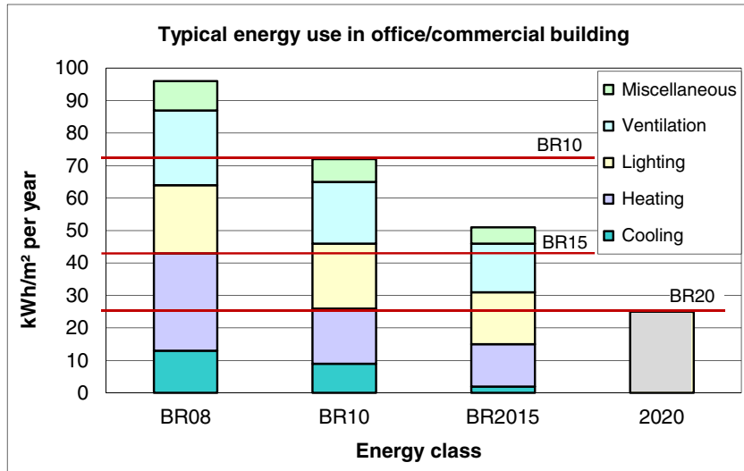
Figure 1. Energy requirements (shown by the horizontal lines) in the Danish building regulations from 2008 till 2020. The first three columns illustrate the typical constituents of the total energy consumption in offices or commercial buildings when using passive façade technologies. The last column shows the 2020 energy demand, which can only be met by dynamic technologies (or by introducing sustainable energy supply). The energy demands must be documented by a standard calculation method, Be10, based on EN ISO 13790 [3].
