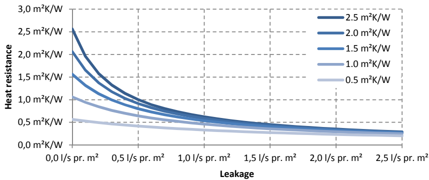
Figure 3. The graph shows the effective heat resistance for different shutter resistances as function of leakage in blower-door test at 50 Pa.
