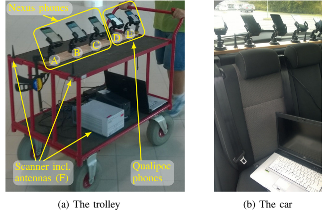
Fig. 3: The measurement tools and transportation devices.
