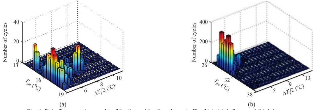
Fig. 6. Rain-flow counting results of the thermal loading shown in Fig. 5(a): (a) Aalborg and (b) Arizona.
