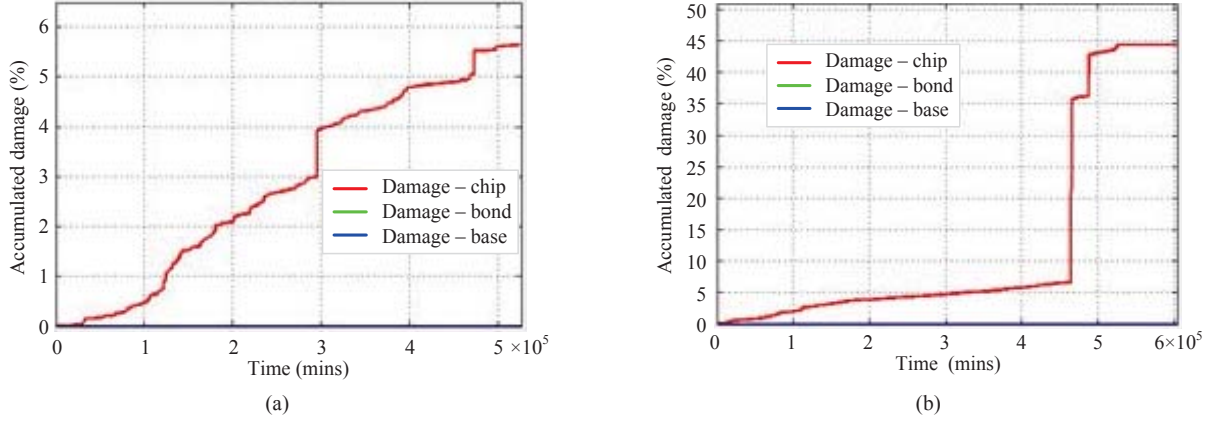
Fig. 7. Accumulated chip, bond (wire), and base damage of the power devices of the PV inverter: (a) in Aalborg and (b) in Arizona.
