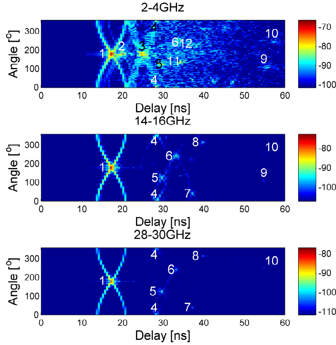
Figure 14. Power-angle-delay profile measured with UCA for LOS scenarios at different frequency bands. The power dynamic range is limited to 35 dB.
