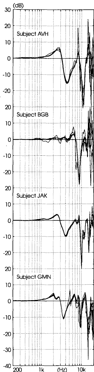
Fig. 17. Examples of pressure division P_3/P_2 for left ears of four subjects. Curves are shown for the five directions ( \phi = 0^\circ, 90^\circ, 180^\circ, \text{ and } -90^\circ in horizontal plane; \theta = 90^\circ ).
