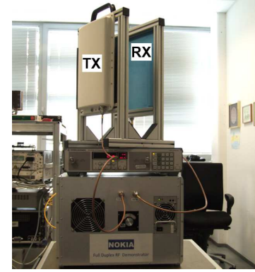
Fig. 3: SIC hardware platform
