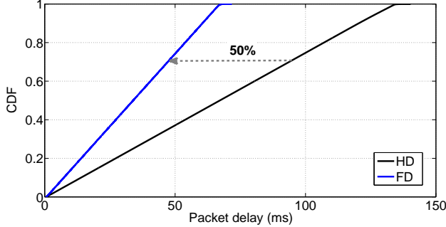
Fig. 7: Single cell delay with 100% FD probability
