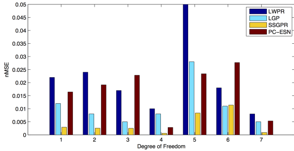
Fig. 5. Evaluation of generalization ability. All algorithms were trained with the Sarcos training set. The illustrated error corresponds to the estimated torques on the testing set. LWPR and LGP results are taken from [11].
