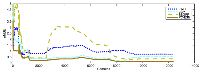
Fig. 7. Torque estimation error on a single joint of the UR10 dataset. Large error fluctuations are caused because of low adaptability.
