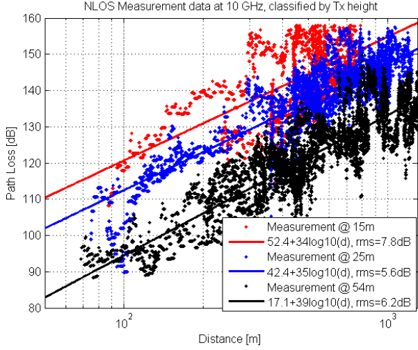
Fig. 4. Measured path loss data for the 10 GHz band at different Tx heights.
