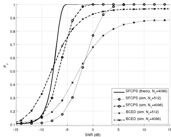
Fig. 3. P_d versus SNR for OFDM signal at P_{fa} = 10\%
