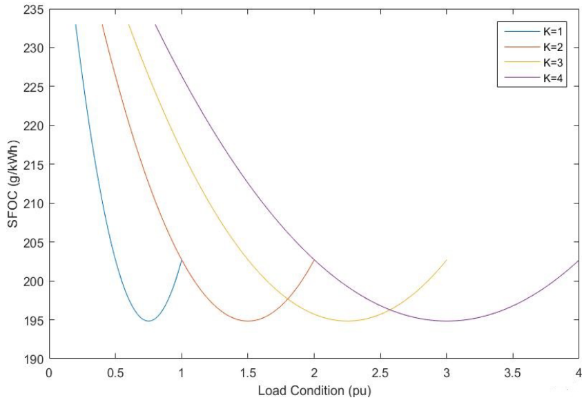
Fig.5 Schematic diagram of fuel efficiency characteristic for diesel generation (in fixed speed)
