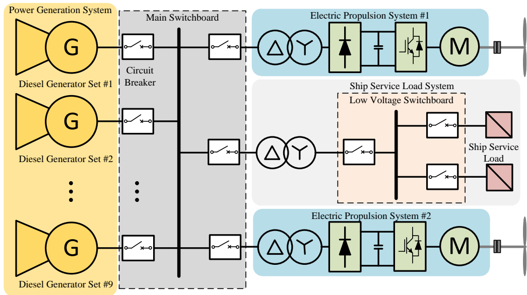
Fig.1 Diesel-Electric Shipboard Power System of the Queen Elizabeth II
