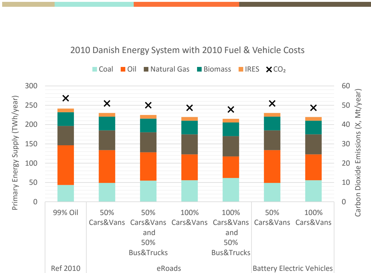
Figure 10: Primary energy supply and carbon dioxide emissions for the Ref 2010 scenario with various penetrations of eRoad and battery electric vehicles, based on the scenarios presented in Table 3 and the eRoad infrastructure proposed in Table 4. The fuel and vehicle costs as based on the year 2010 (see Table 6).
