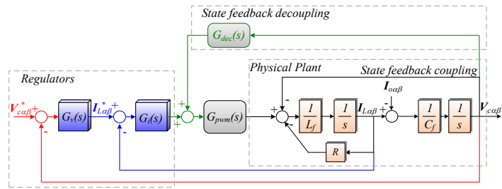
Fig. 2. Simplified state block diagram of the closed-loop system
