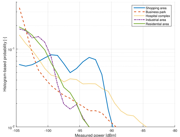
Fig. 7. Received power level probability density function based on a normalized histogram of the measurements in the 868.0-868.6 MHz band.
