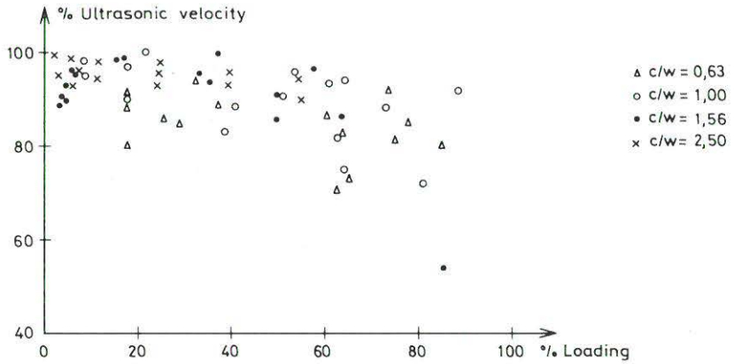
Figure 4: Ultrasonic velocity (%) versus loading.
