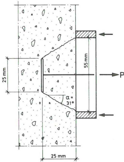
Figure 1: Lok-test sketch.
