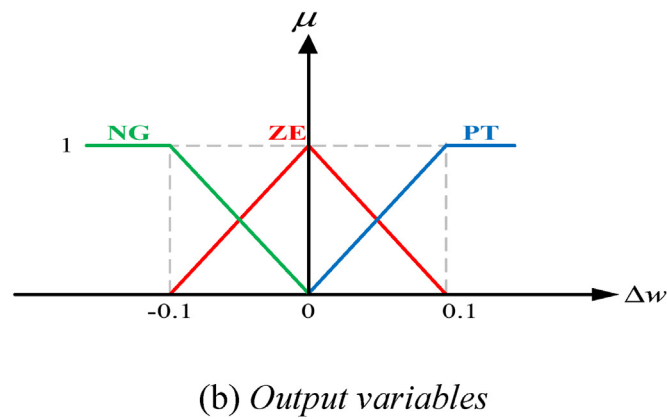
Fig. 4. Fuzzifiers for the inertia weight correction factor.
