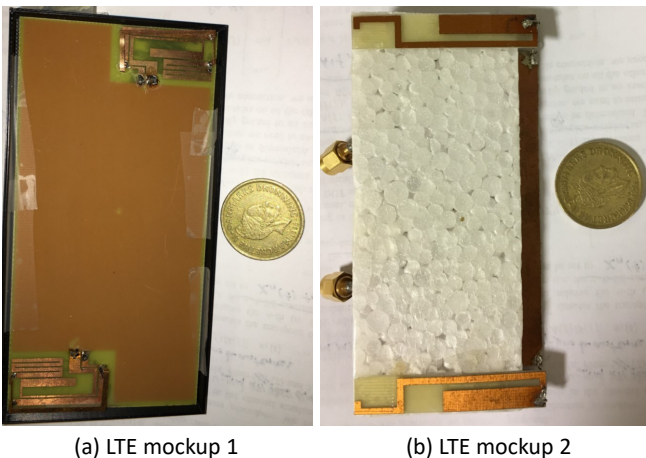
Figure 6. A photo of the two LTE mockups.
