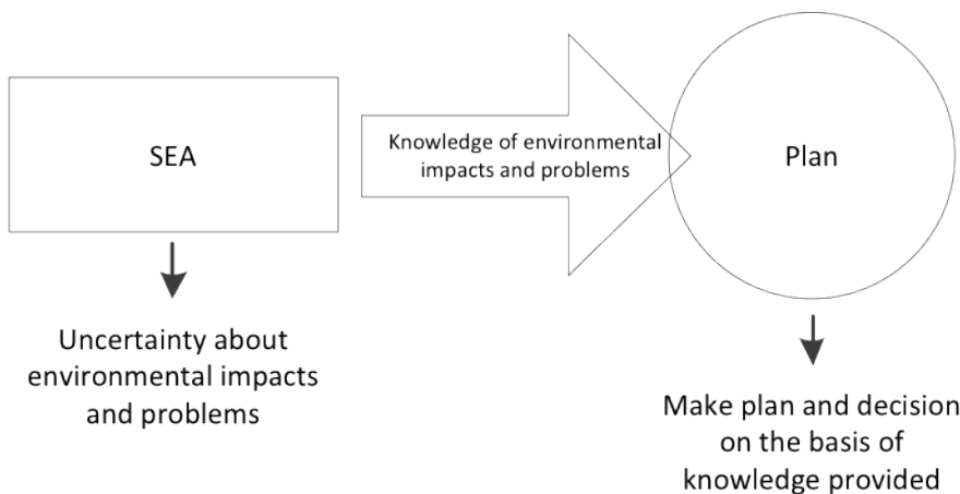
Figure 3: The simplified relations between SEA, plan and uncertainty
