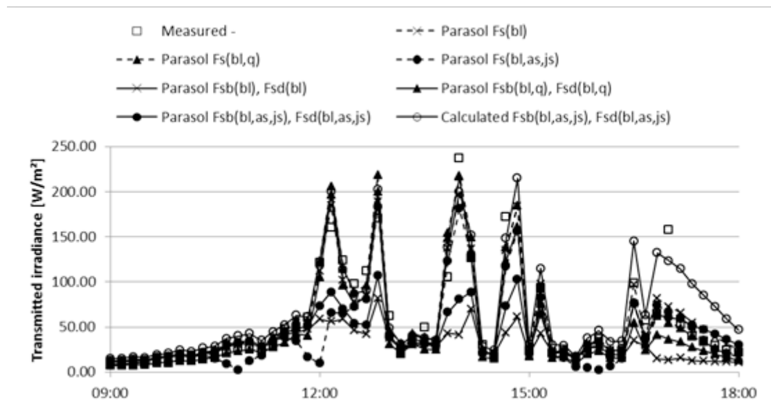
Fig. 4. Calculated and simulated transmitted irradiance for a slat angle of 0^\circ for the 29/3-11.
