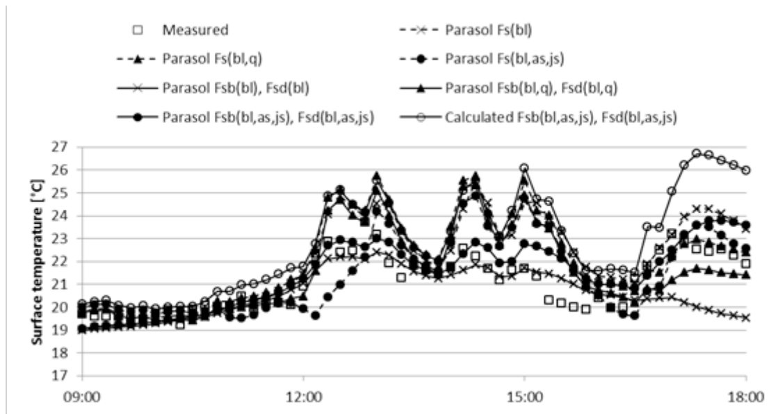
Fig. 3. Calculated and measured surface temperature of glazing system for a slat angle of 0^\circ 29/3-11.
