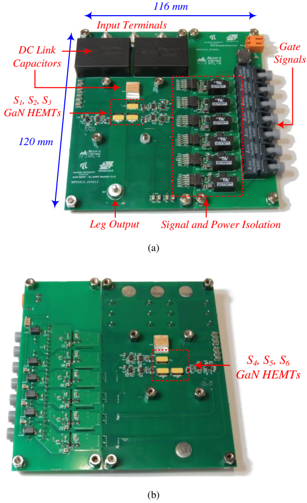
Fig. 12: Hardware of the GaN HEMT based single-phase 3L-ANPC power cell: (a) top view and (b) bottom view.
