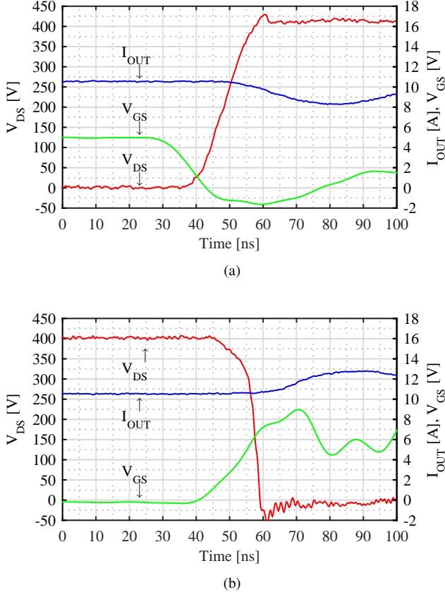
Fig. 16: Switching waveforms of S_1 in the commutation loop presented in Fig. 5b for: (a) turn-off and (b) turn-on.
