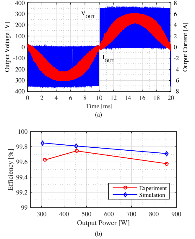
Fig. 18: (a) Experimental output voltage and current waveforms at 800 W output power and (b) efficiency of the 3L-ANPC power cell with experimental and simulation results.
