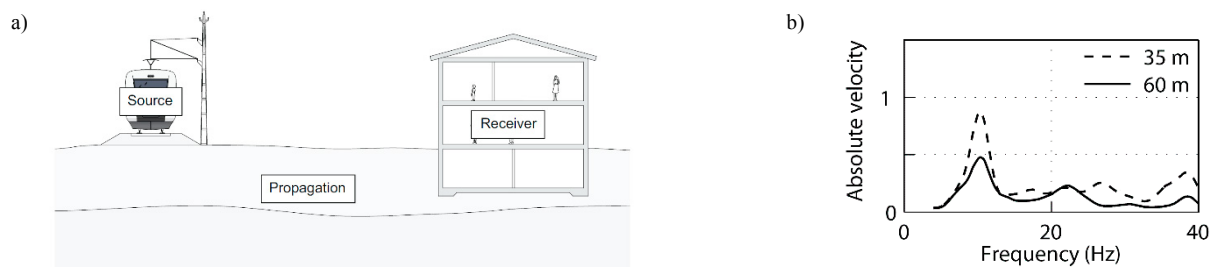
Fig. 1. a) Illustration of the vibration propagation problem. b) Example of measured ground velocity response caused by passing freight train, evaluated 35 and 60 m from the track, respectively [5].
