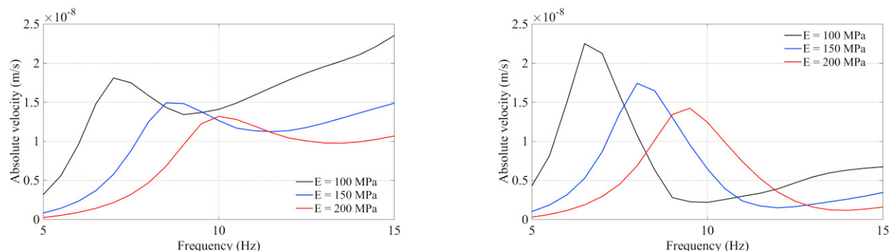
Fig. 4. Vibrations evaluated for the concrete building with slab thickness of 0.30 m on soils with different Young's modulus: 100 MPa; 150 MPa; 200 MPa. a) on the ground surface just in front of the building; b) on the top floor.
