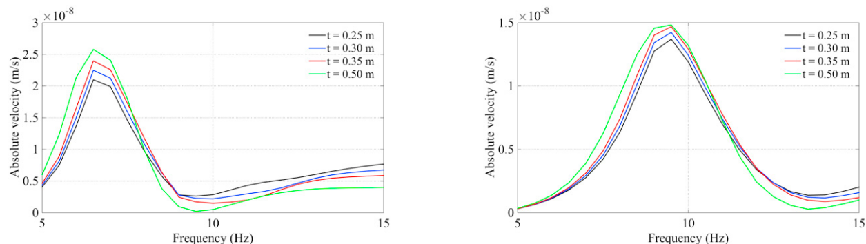
Fig. 5. Vibrations evaluated on the top floor of the concrete building for two types of soils: a) E = 100 MPa and b) E = 200 MPa. The thickness of the slabs were varied from 0.25 to 0.50 m. Note that the vertical scale of the figures is not identical.
