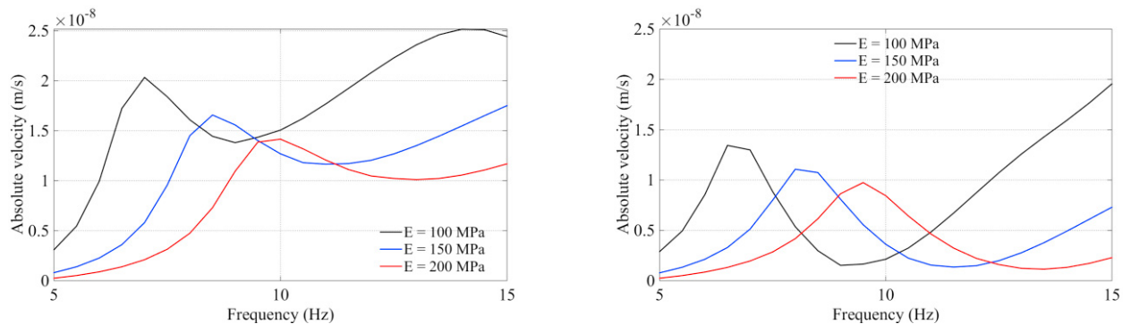
Fig. 6. Vibrations evaluated for the wooden structure with slab thickness of 0.24 m on soils with different Young's modulus: 100 MPa; 150 MPa; 200 MPa. a) on the ground surface just in front of the building, b) on the top floor.
