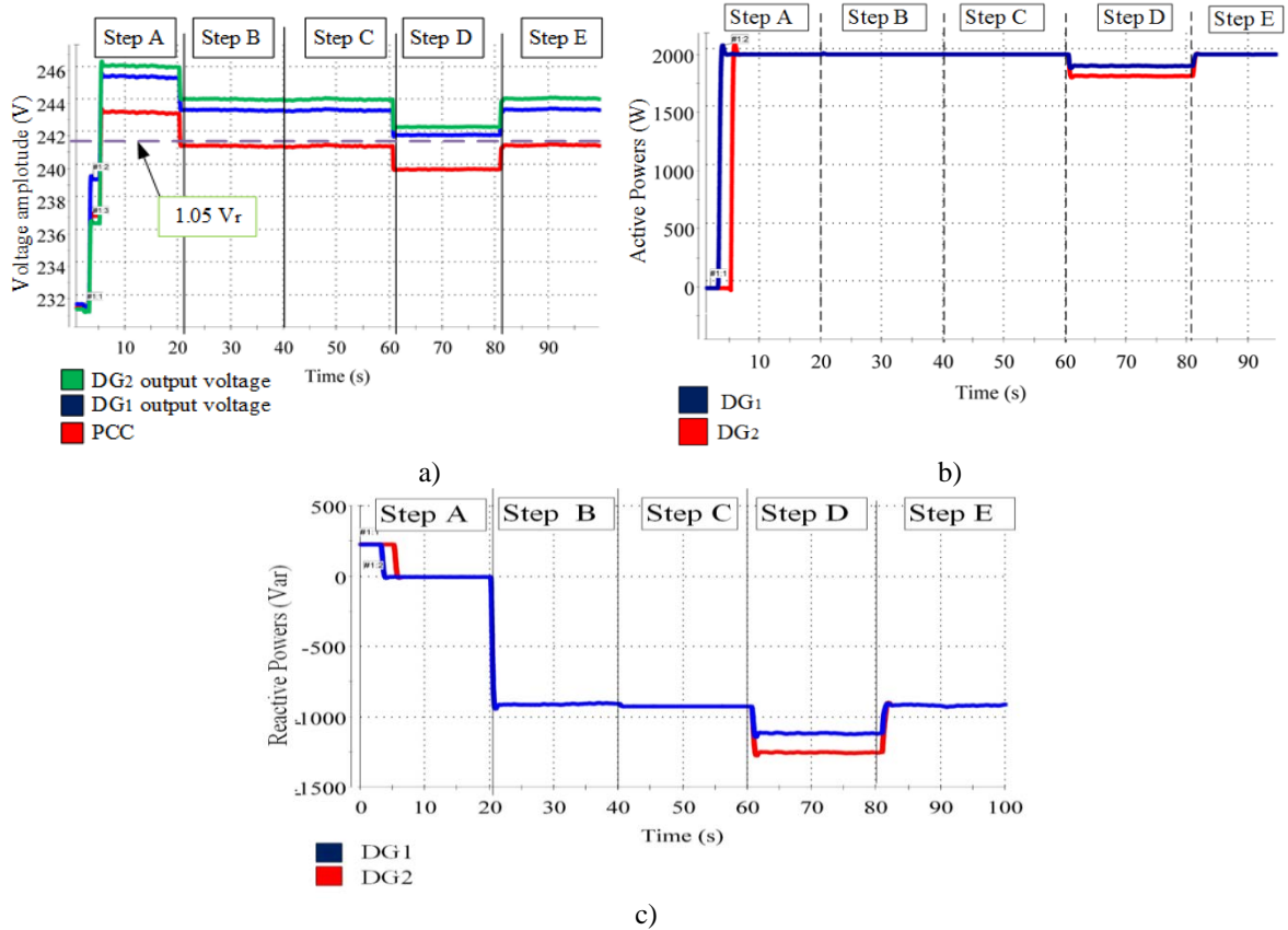
Fig. 11. Experimental results in second scenario with 231 V grid voltage , a) voltage amplitude, b) active power, c) reactive power
