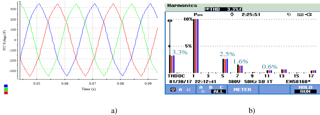
Fig. 14. PCC voltage, with communication system and 5ms delay in third scenario (Experimental results) a) voltage waveform, b) harmonic content
