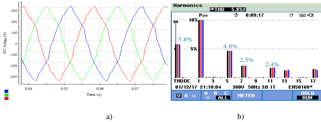
Fig. 13. PCC voltage before harmonic compensation in third scenario (Experimental results), a) voltage waveform, b) harmonic content
